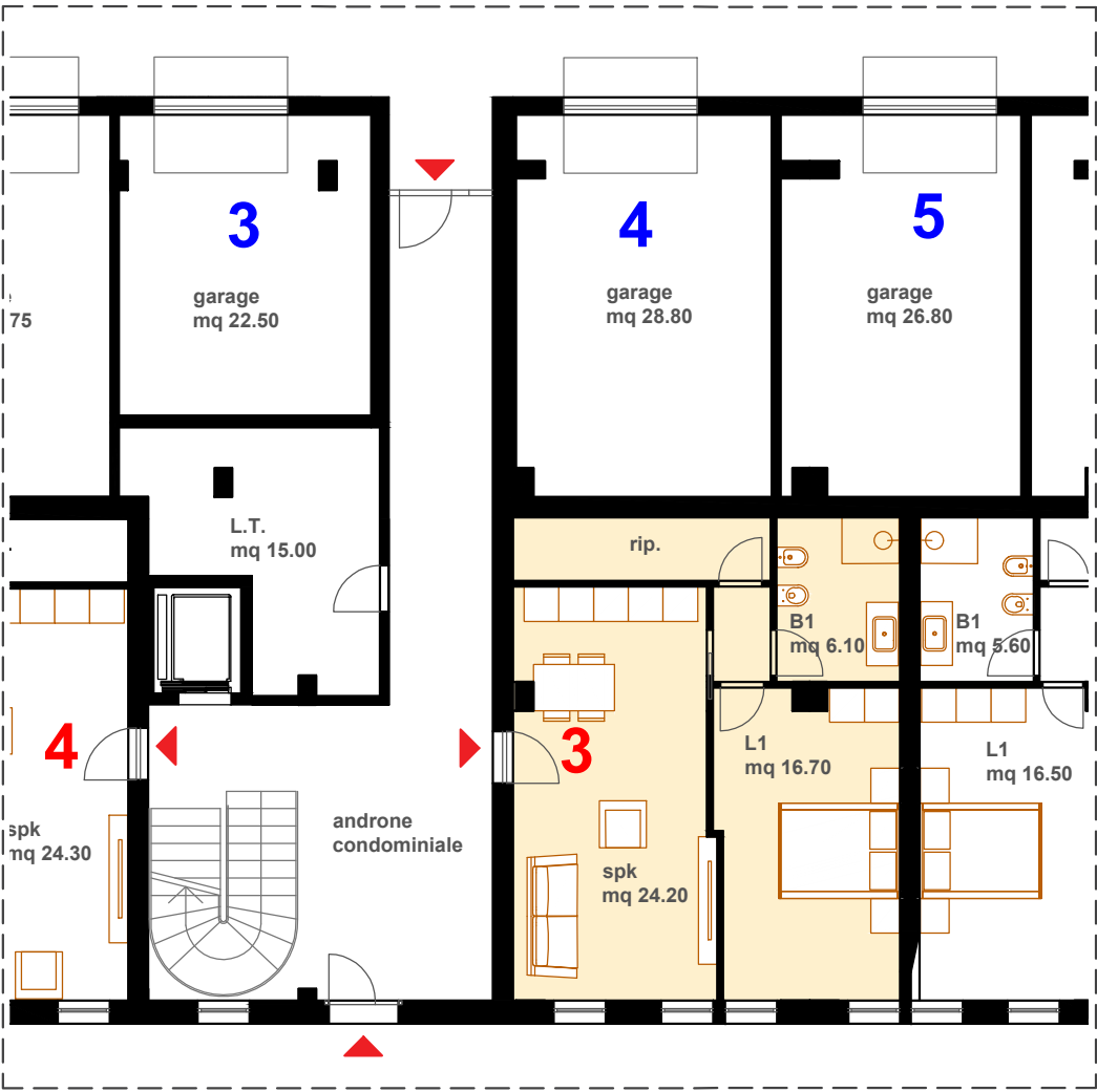
Planimetria piano terra
